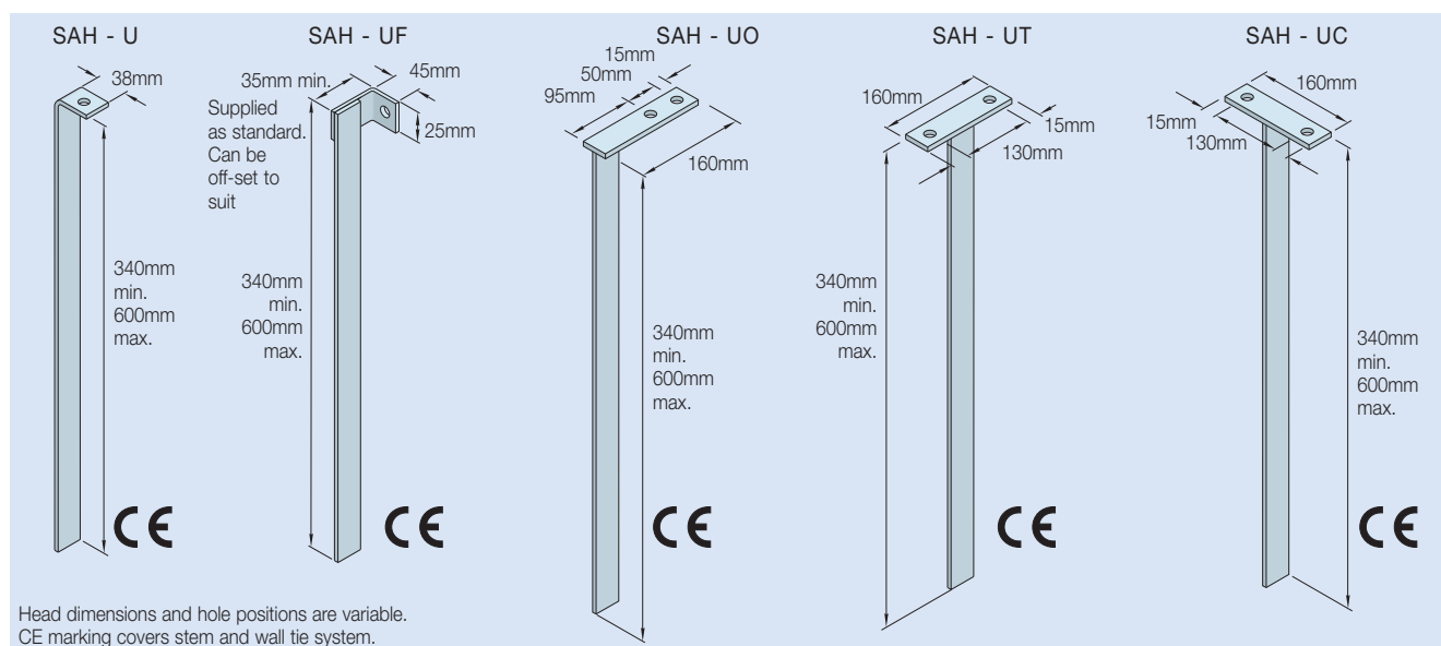
These drawings are examples only. All sliding anchors are manufactured to suit individual requirements.
