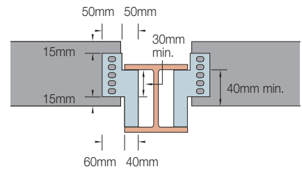
Non-Standard Internal Column Tie
